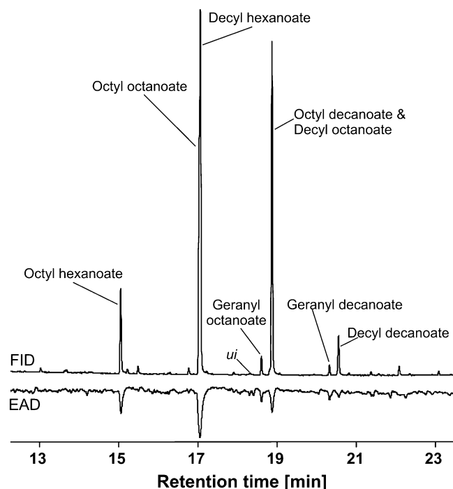
Figure 3 Gas chromatogram (FID) of a labial gland extract from a Trigona corvina forager and simultaneous recording of the chemoreceptors' responses (EAD) of an antenna from a worker taken from the same nest. Names of physiologically active compounds are given in the chromatogram. ui, unidentified compound (=peak 10 in Figure 2).
